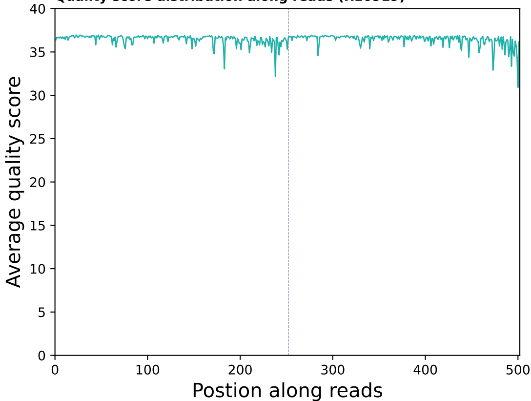
Quality score distribution along reads (R10919)
